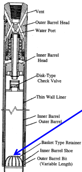
Denison Double-Tube Core Barrel Soil Sampler (Courtesy of Sprague & Henwood, Inc.)
